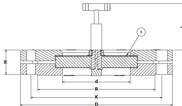
Flanged (F)
